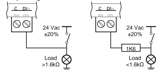
Example wiring
